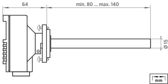
GMD20 Dimensions
