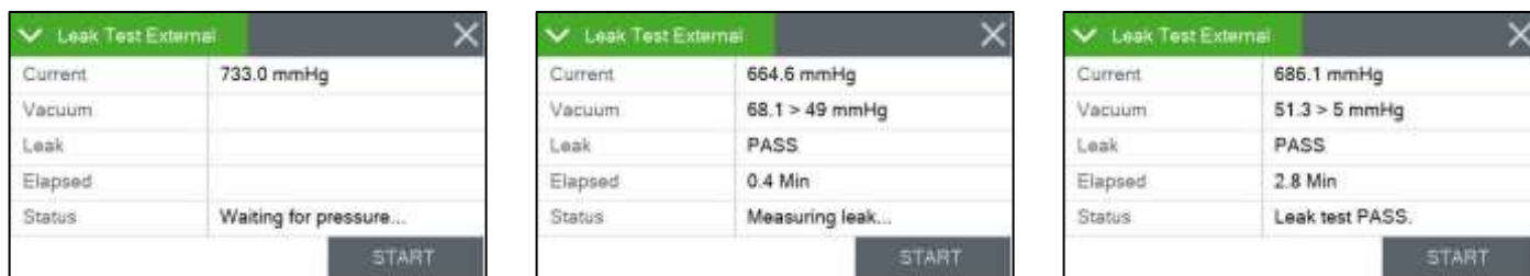
Figure 6-3 External Leak Test Sequence
