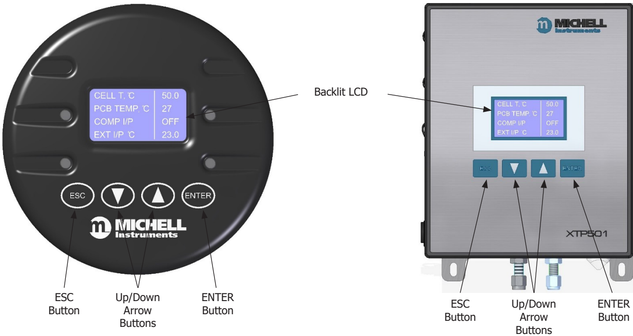
Figure 4 User Interface
