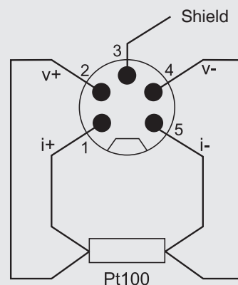
4-wire PRT connection
