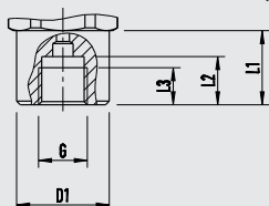
EN 837, female thread, Ermeto-compatible
