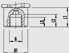
EN 837, female thread
